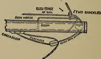
GEAR FOR HAULING OUT LOOSE-FOOTED MAINSAIL.
